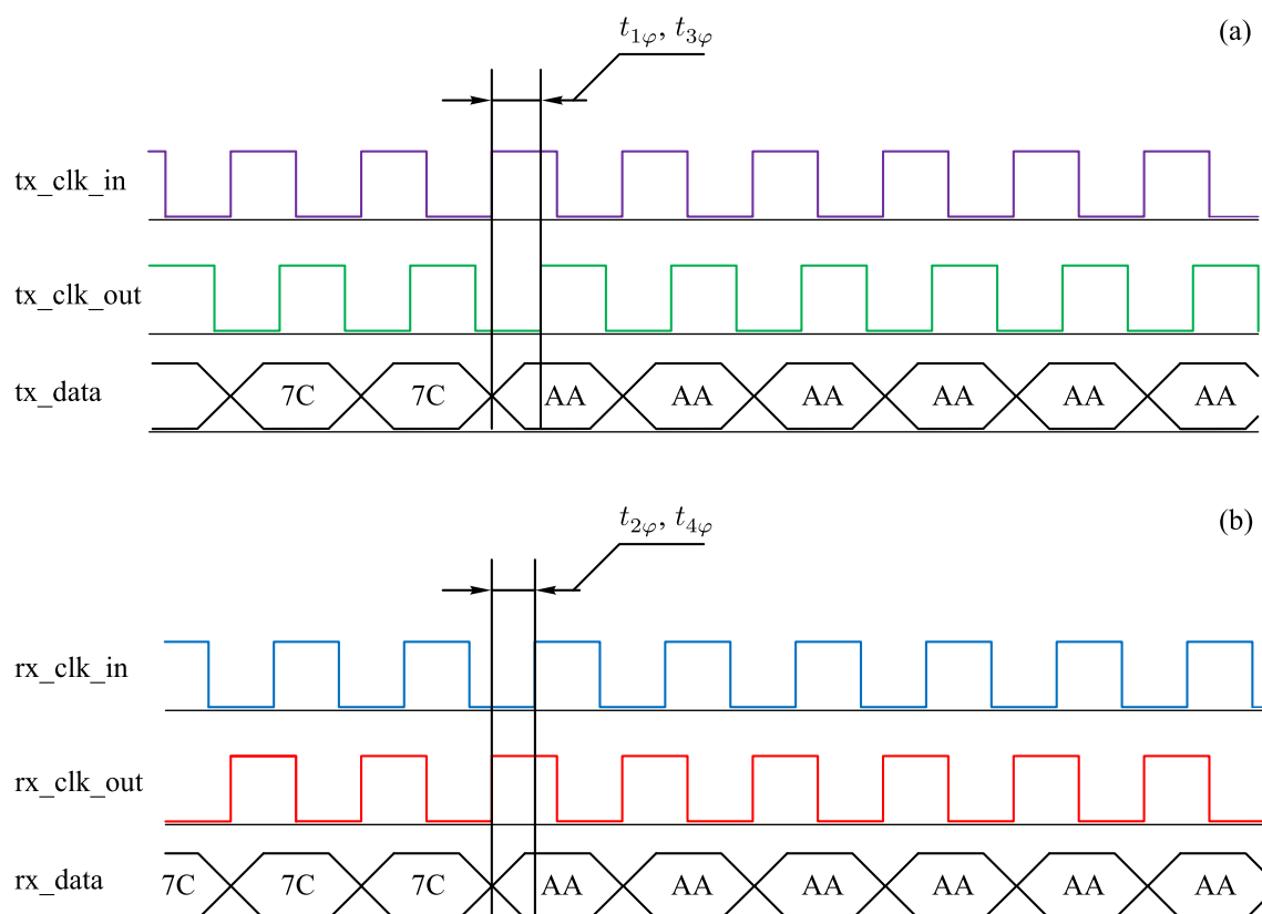
Figure 6. To account for the phase difference in the time stamps of receive and transmission. For rx packet timestamps, the phase is fixed with a minus sign. For tx packet timestamps, the phase value is fixed with a plus sign
