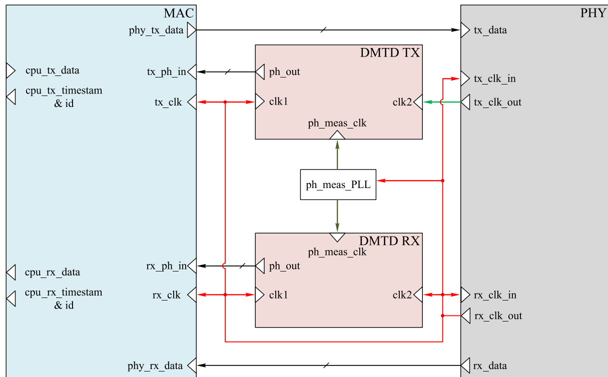
Figure 5. A modified MAC and PHY connection scheme, provides subnanosecond timing accuracy for the two-way synchronization method
