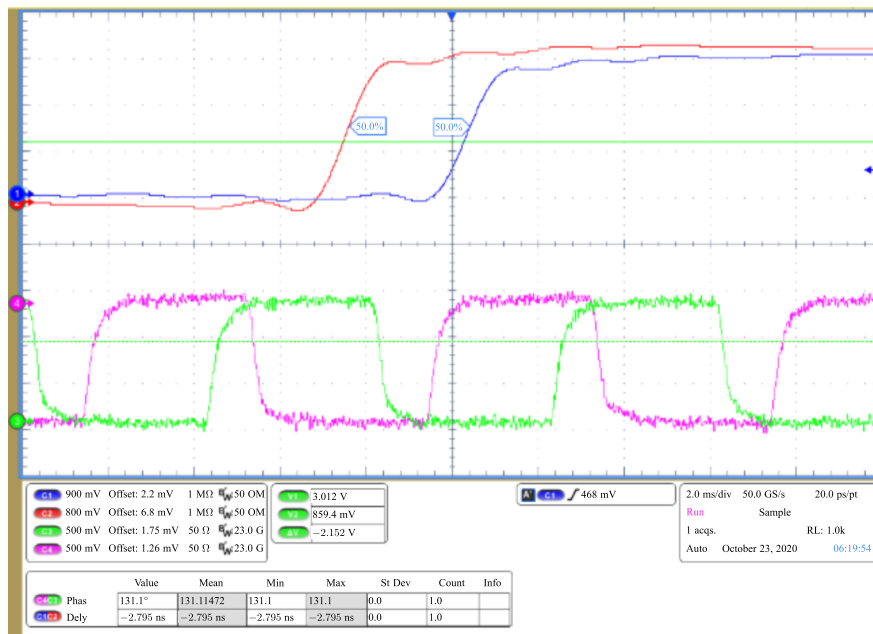
Figure 11. Synchronization result before phase compensation. There is a significant timing error, about 3 ns, as well as a significant phase difference between the device clocks
