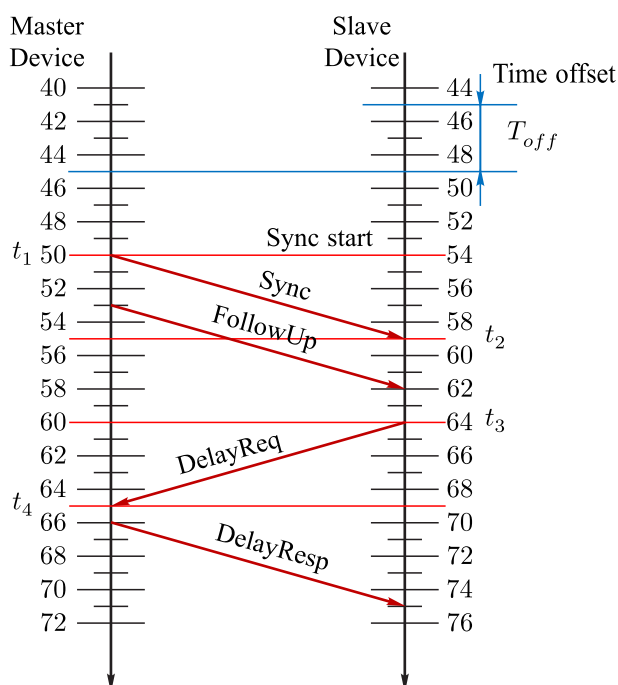
Figure 2. The process of exchanging messages between devices using the classic two-way synchronization method
