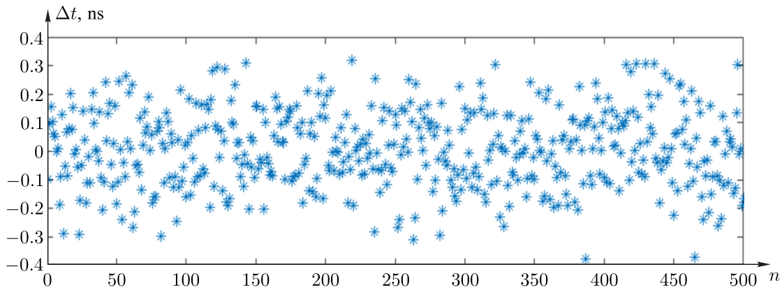
Figure 13. Synchronization error against synchronization cycle number
