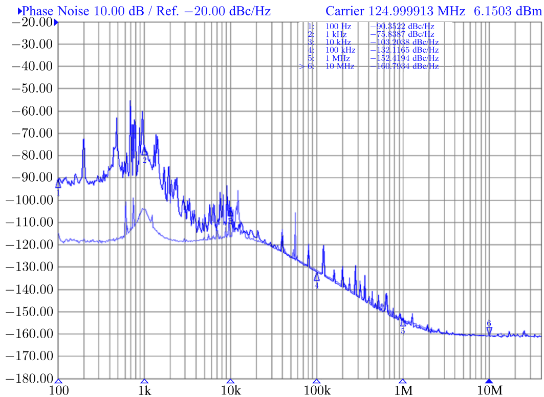
Figure 9. Graph of the spectral density of phase noise in sections 2 (bottom) and 4 (top). There is a significant suppression of phase noise at the output of the PLL in the region of large frequency offsets
