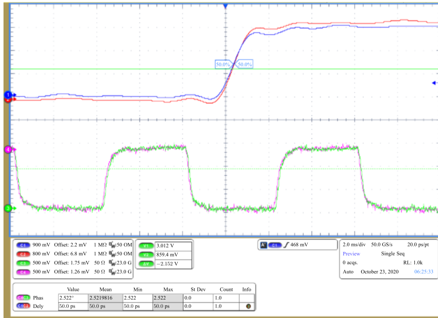
Figure 12. Synchronization result after phase compensation. There is precise synchronization of the PPS signals, as well as precise alignment of the clock signals of the devices
