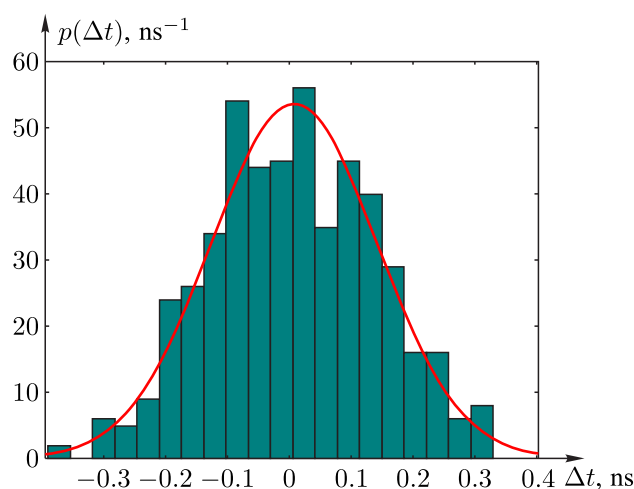
Figure 14. Distribution law of synchronization error
