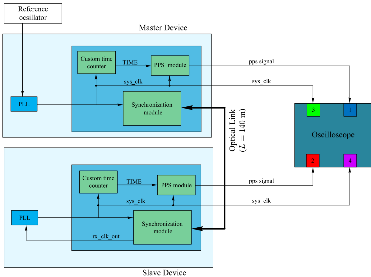
Figure 10. Simplified block diagram of the stand for estimating synchronization accuracy
