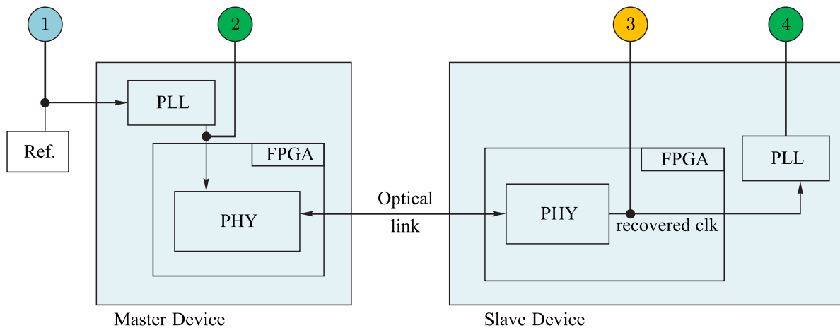
Figure 7. Simplified block diagram of the experiment to determine the phase noise of the clock signal, restored from the data
