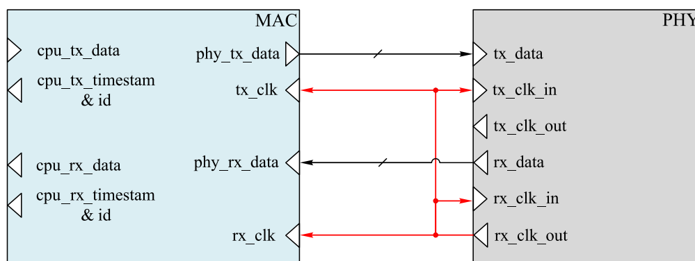
Figure 4. Standard MAC and PHY connection scheme, provides basic timing accuracy for the two-way synchronization method
