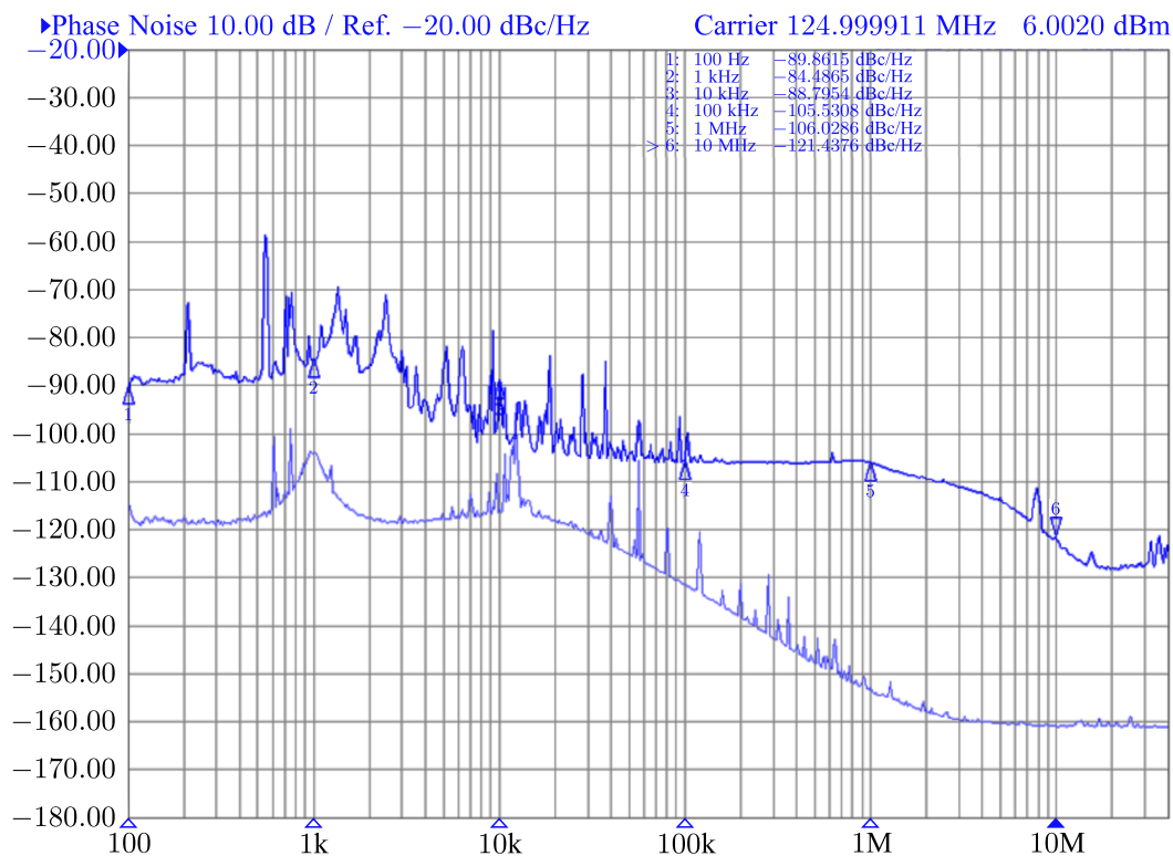
Figure 8. Graph of the spectral density of phase noise in sections 2 (bottom) and 3 (top). There is a significant increase in the phase noise level of the recovered clock signal at the CDR output
