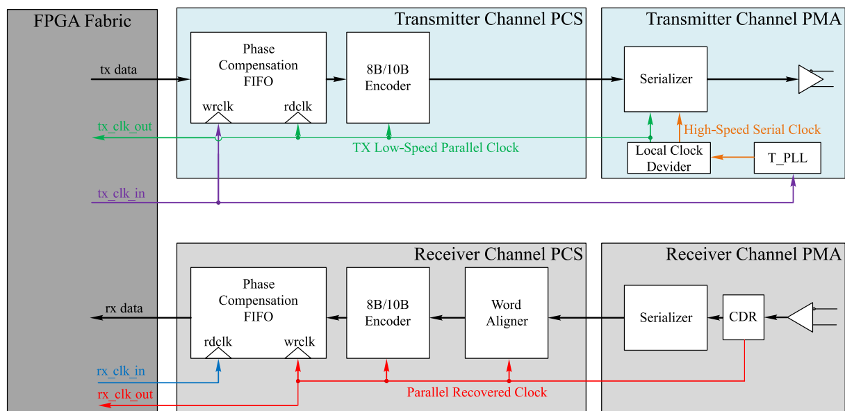
Figure 3. FPGA Transceiver unit configuration for constant transmit and receive delays
