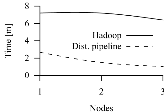
Fig. 2. Performance of Hadoop and distributed pipeline implementations
